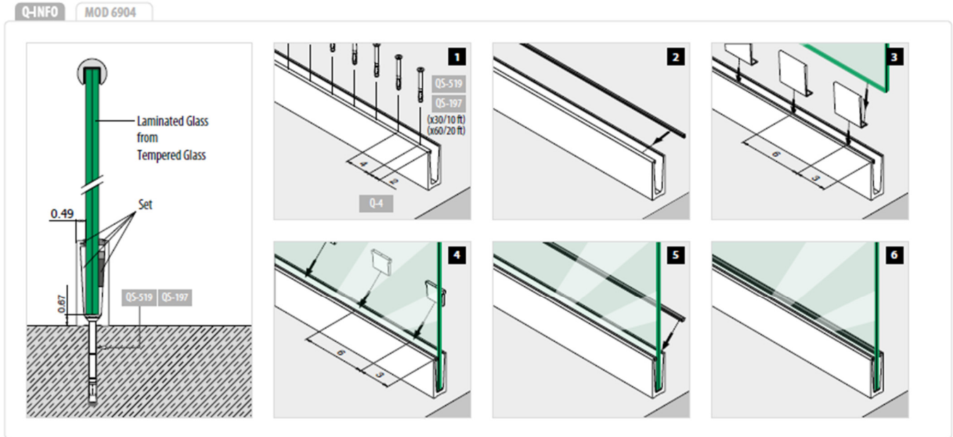
FIGURE 2—GUARD RAIL ASSEMBLY COMPONENTS (WEDGE SYSTEM)
