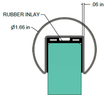
Ø 1.66 in CAP RAIL - ROUND MAT.: SS 304, SS 316
