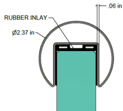
Ø 2.37 in CAP RAIL - ROUND MAT.: SS 304, SS 316
