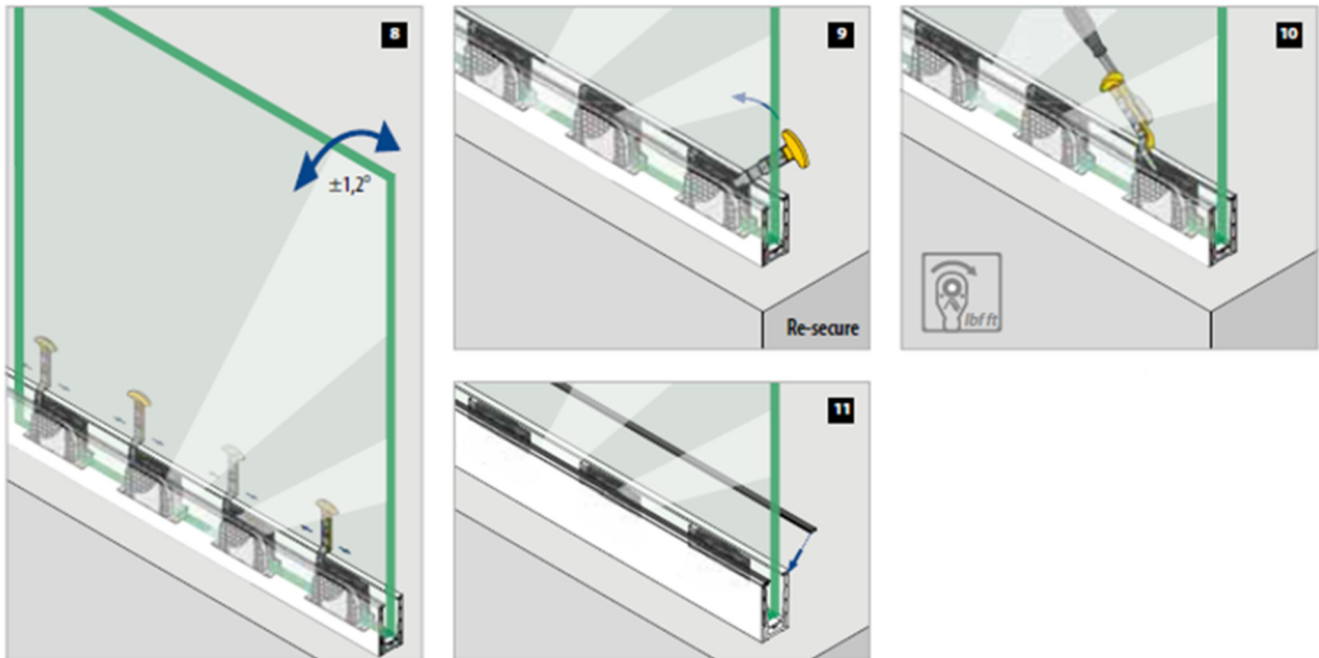
FIGURE 3 (CONT'D)—GUARD RAIL ASSEMBLY COMPONENTS (Q-DISK SYSTEM)
