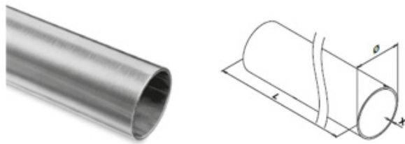
MOD 8925 / 0900 Ø 1-1/2" (38.1 mm)
