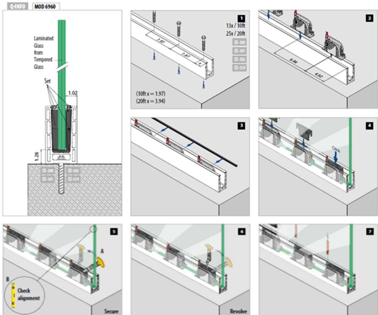
FIGURE 3—GUARD RAIL ASSEMBLY COMPONENTS (Q-DISK SYSTEM)
