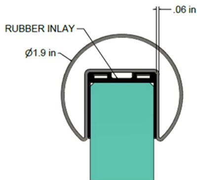
Ø 1.9 in CAP RAIL - ROUND MAT.: SS 304, SS 316
