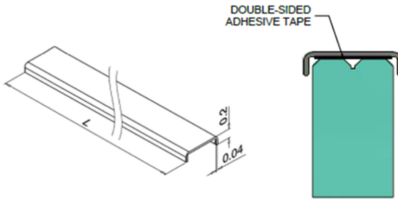
MOD 6940 (EDGE PROTECTION, RECTANGULAR, SS 316) (GLASS THICKNESS: 1/2" - 27/32")
